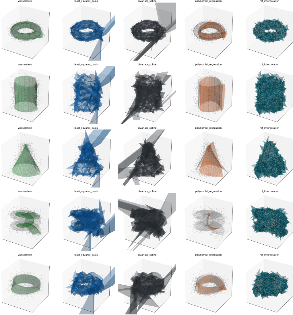
Figure 4: Surface comparison panels corresponding to the last five rows of Table 3: torus, cylinder, cone, helicoid, and Mobius strip.
